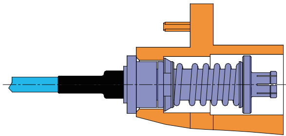
VITA 67.3 Backplane SMPM Contact
