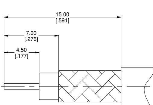
CABLE STRIPPING DIMENSIONS
