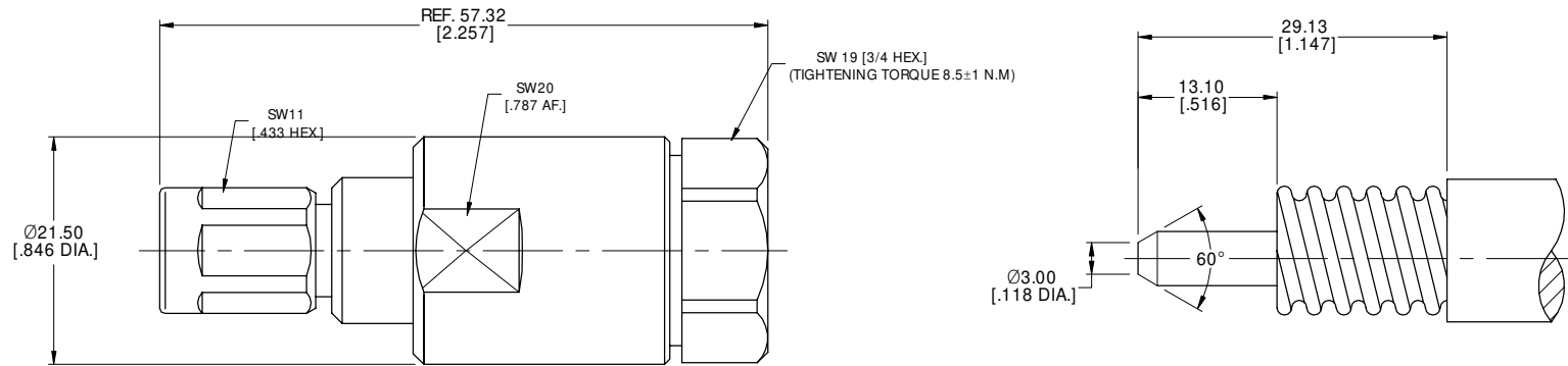
CABLE STRIPPING DIMENSIONS
