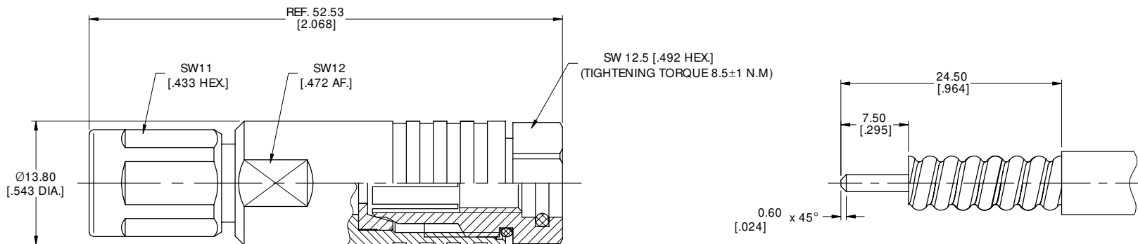
CABLE STRIPPING DIMENSIONS
