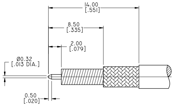
CABLE STRIPPING DIMENSIONS
