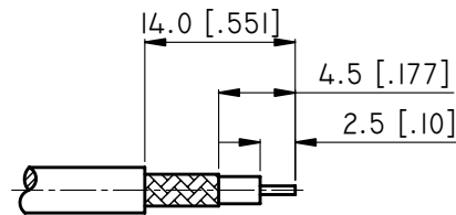
CABLE STRIPPING DIMENSIONS
