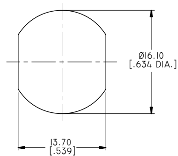
RECOMMENDED PANEL MOUNTING HOLE
