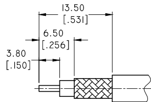
CABLE STRIPPING DIMENSIONS
