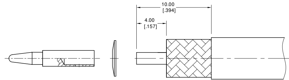
CABLE STRIPPING DIMENSIONS
