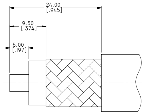
CABLE STRIPPING DIMENSIONS
