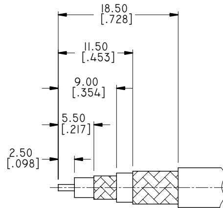
CABLE STRIPPING DIMENSIONS
