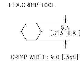
HEX. CRIMP TOOL
