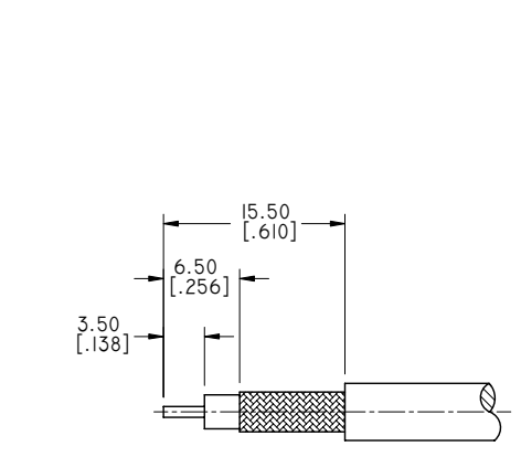
CABLE STRIPPING DIMENSIONS
