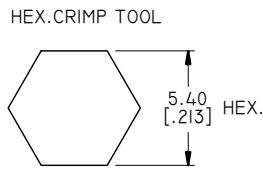
CRIMP WIDTH: 10 [.394]
