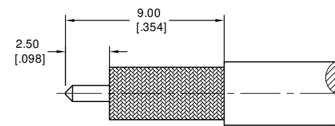
CABLE STRIPPING DIMENSIONS
