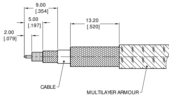
CABLE & MULTILAYER ARMOUR STRIPPING DIMENSIONS
