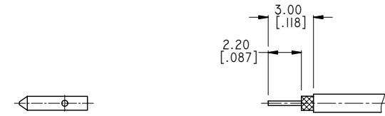
CABLE STRIPPING DIMENSIONS
