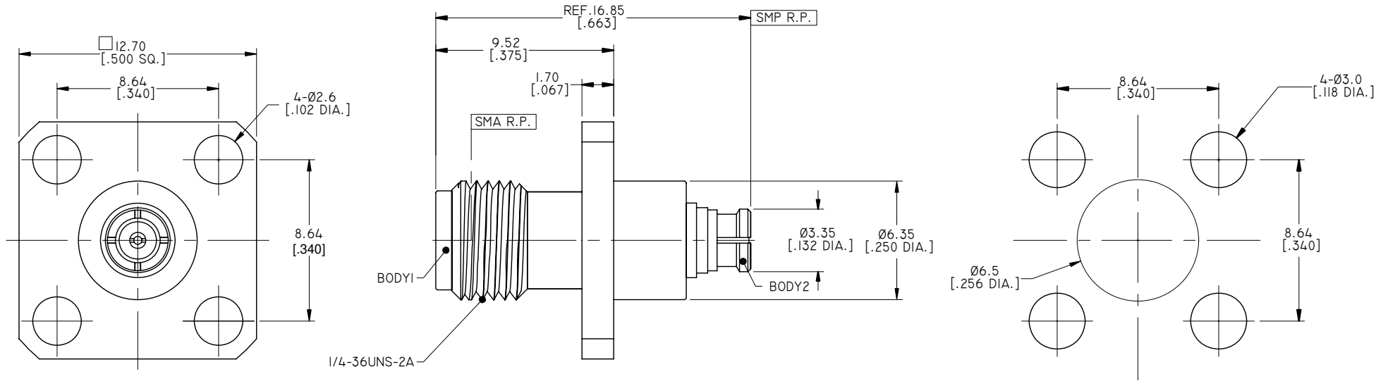
RECOMMENDED MOUNTING HOLE
