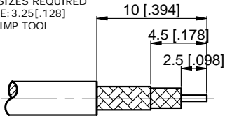
CABLE STRIPPING DIMENSIONS
